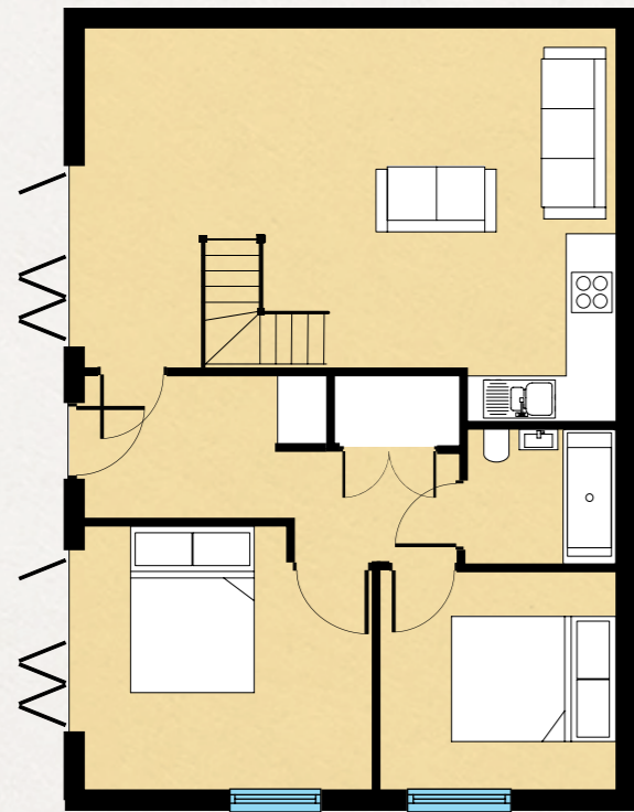
GROUND LEVEL
