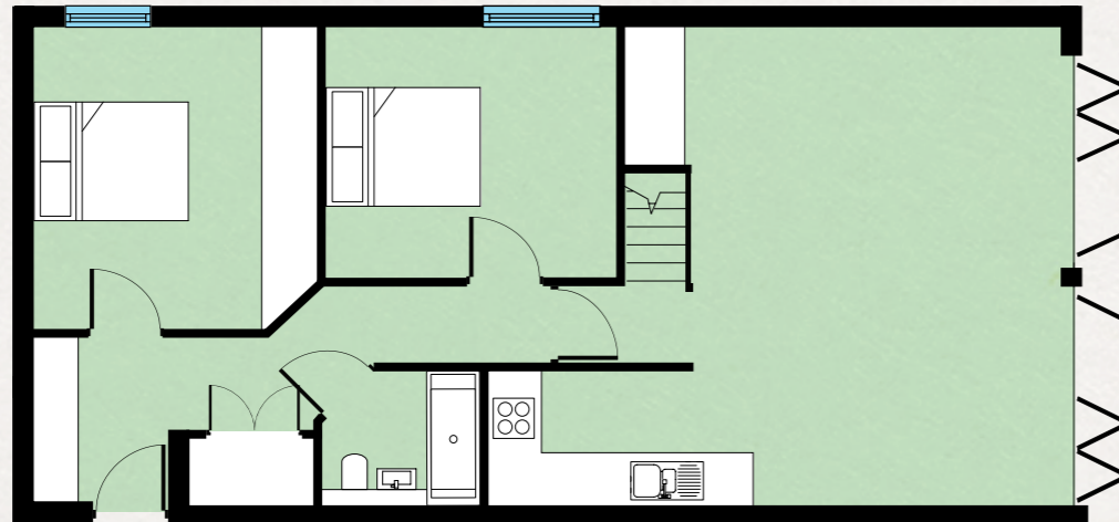
GROUND LEVEL
