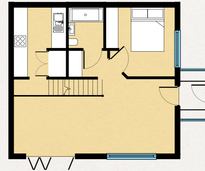
GROUND LEVEL
