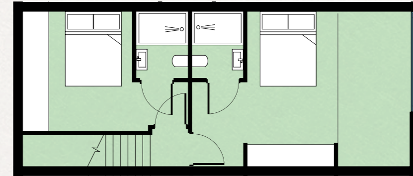
UPPER LEVEL
